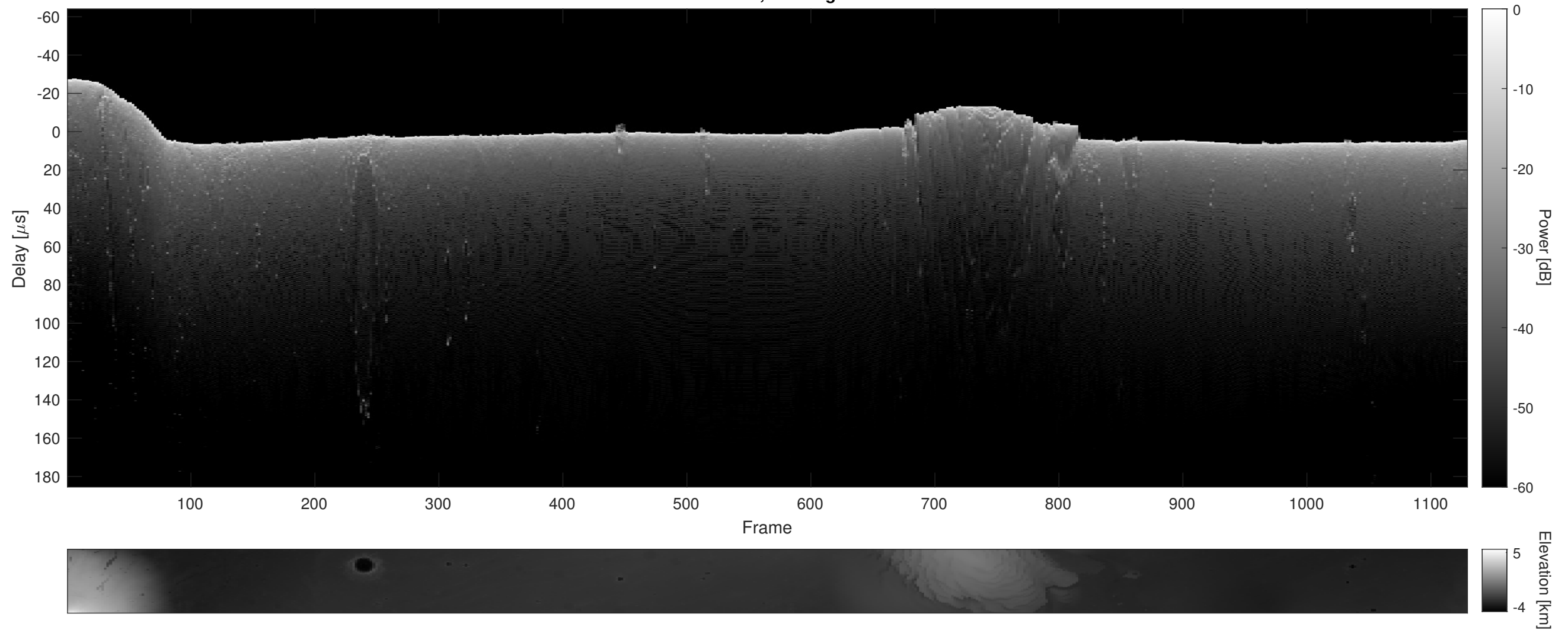
Orbit 11960, Cluttergram
