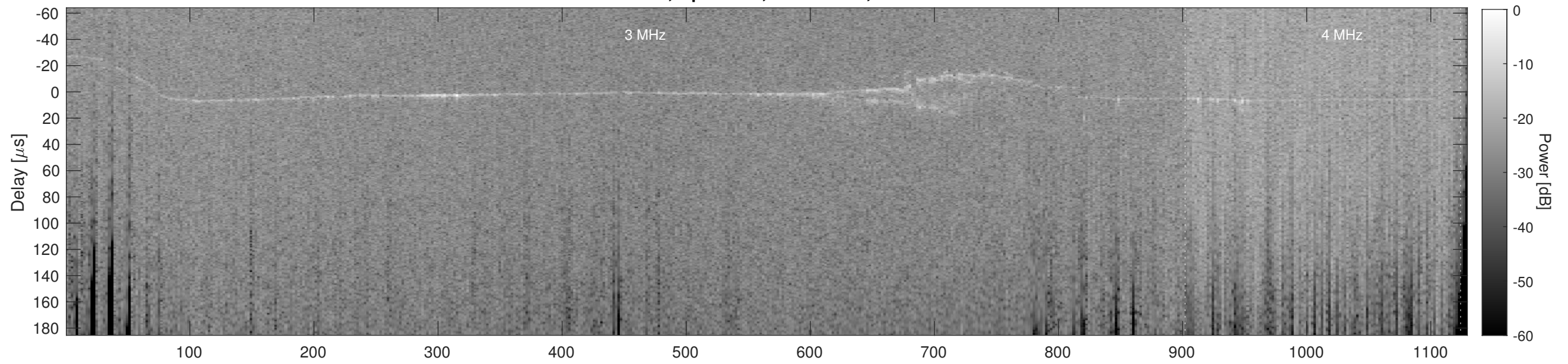
Orbit 11960, Cluttergram
