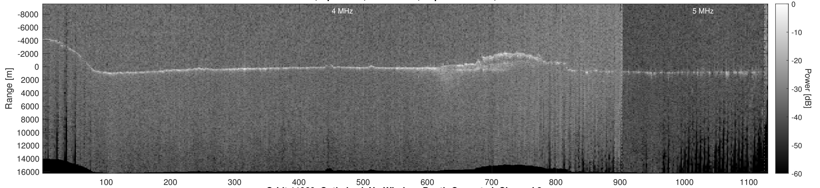
Orbit 11960, Optimized, No Window, Depth-Corrected, Channel 2
