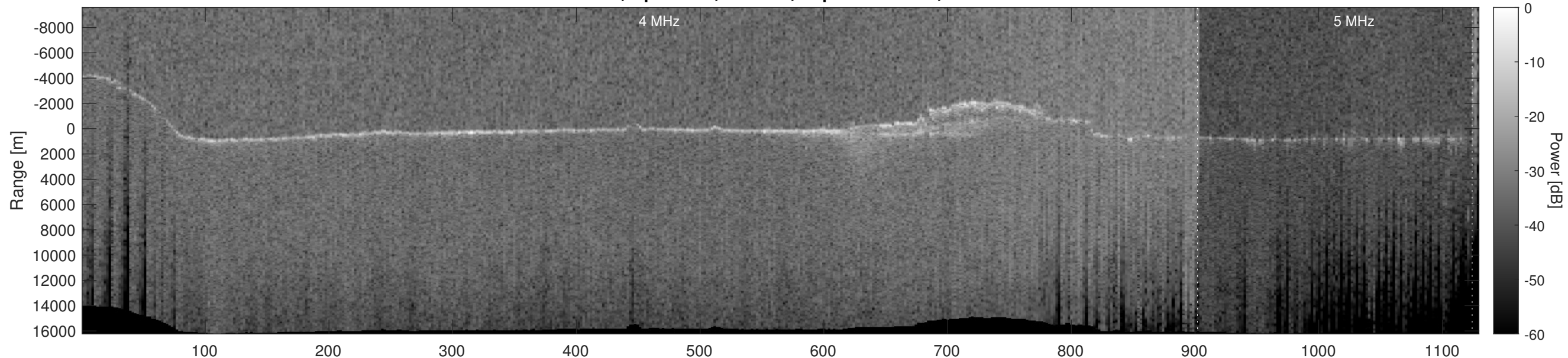
Orbit 11960, Optimized, Window, Depth-Corrected, Channel 2
