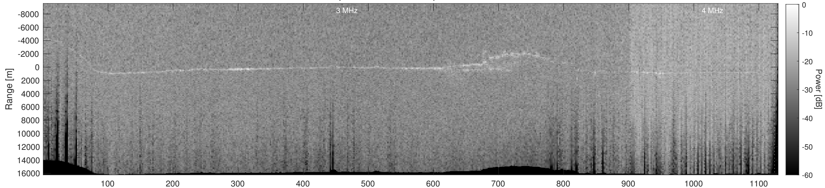
Orbit 11960, Depth-Corrected Cluttergram
