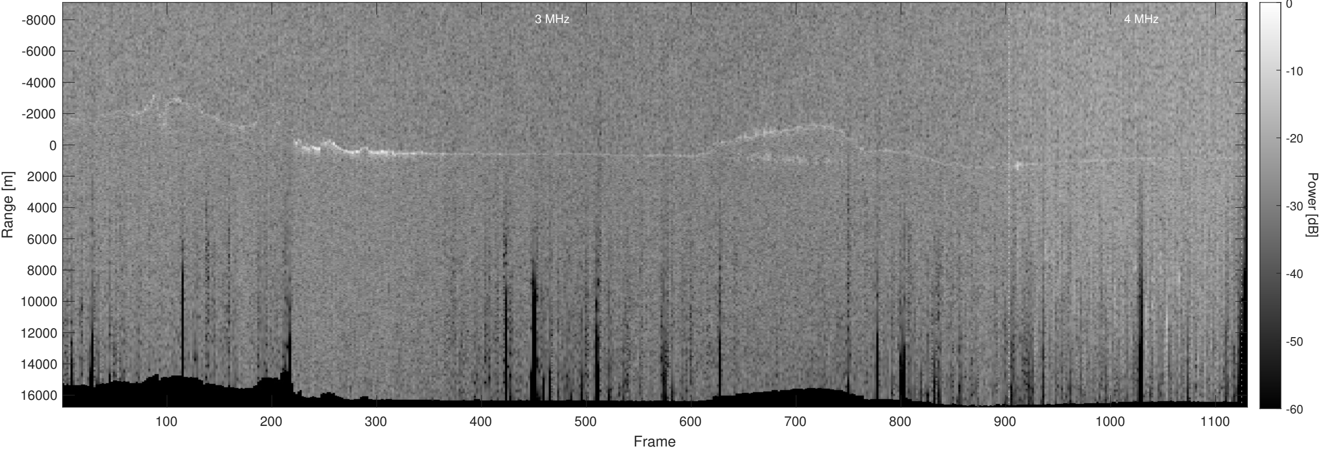
Orbit 11961, Optimized, No Window, Depth-Corrected, Channel 2
