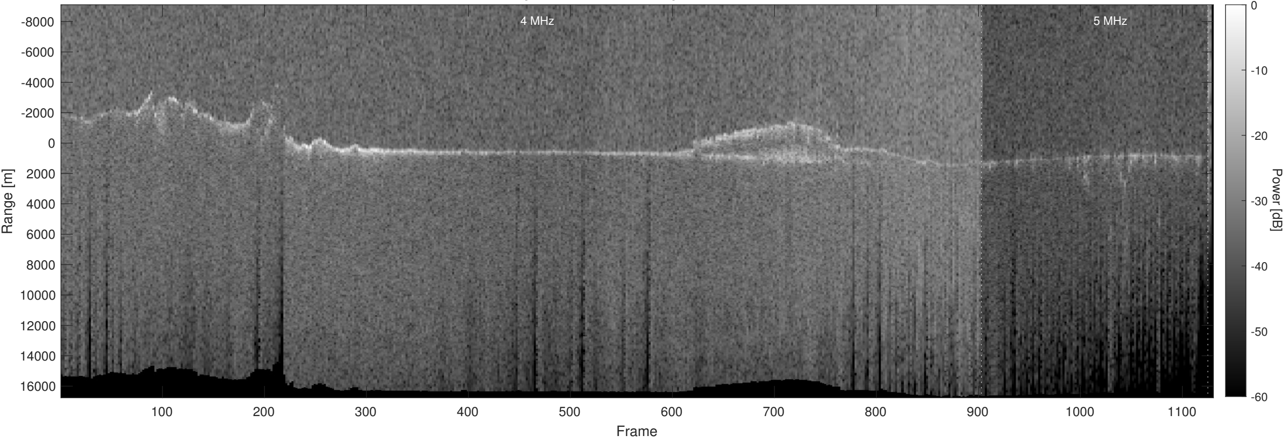
Orbit 11961, Optimized, Window, Depth-Corrected, Channel 2
