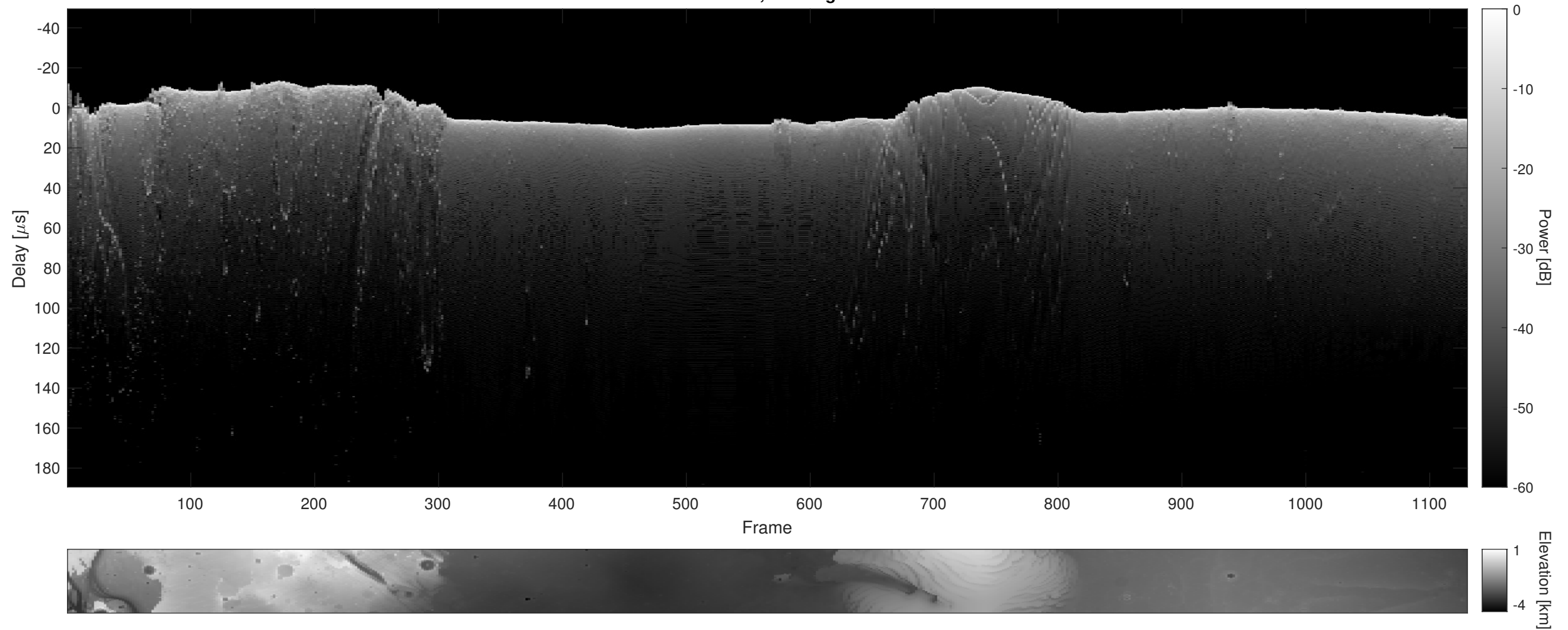
Orbit 11962, Cluttergram
