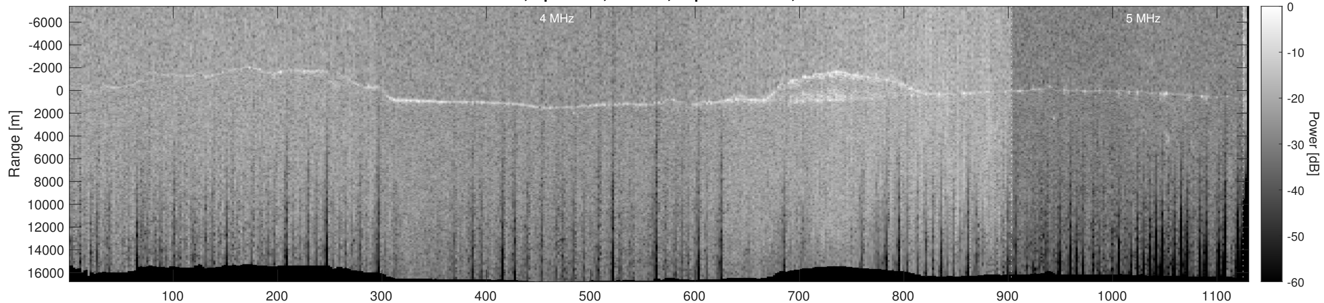
Orbit 11962, Optimized, Window, Depth-Corrected, Channel 2
