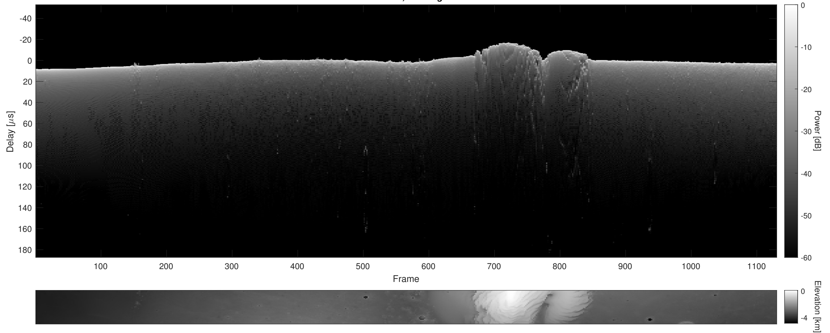
Orbit 11963, Cluttergram
