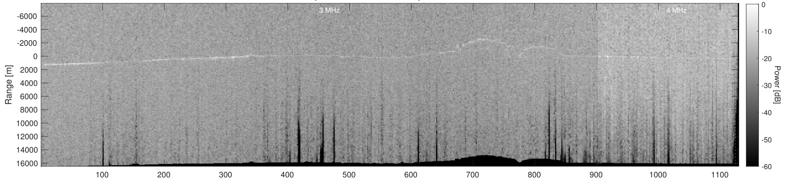
Orbit 11963, Depth-Corrected Cluttergram
