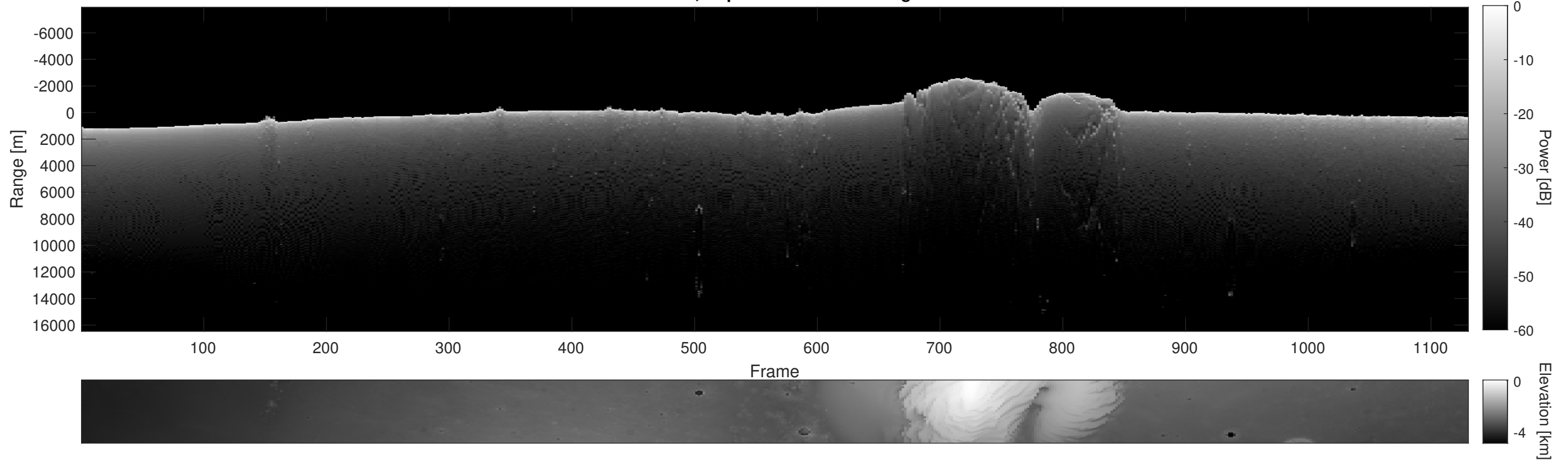
Orbit 11963, Depth-Corrected Cluttergram
