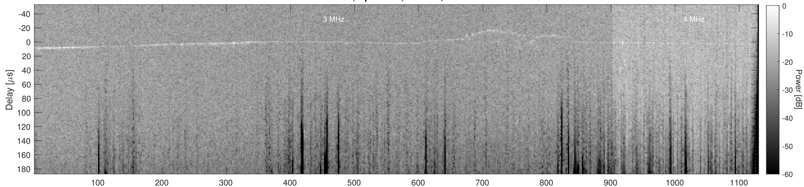
Orbit 11963, Cluttergram
