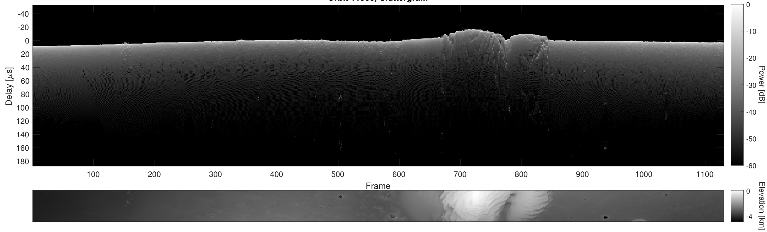
Orbit 11963, Cluttergram
