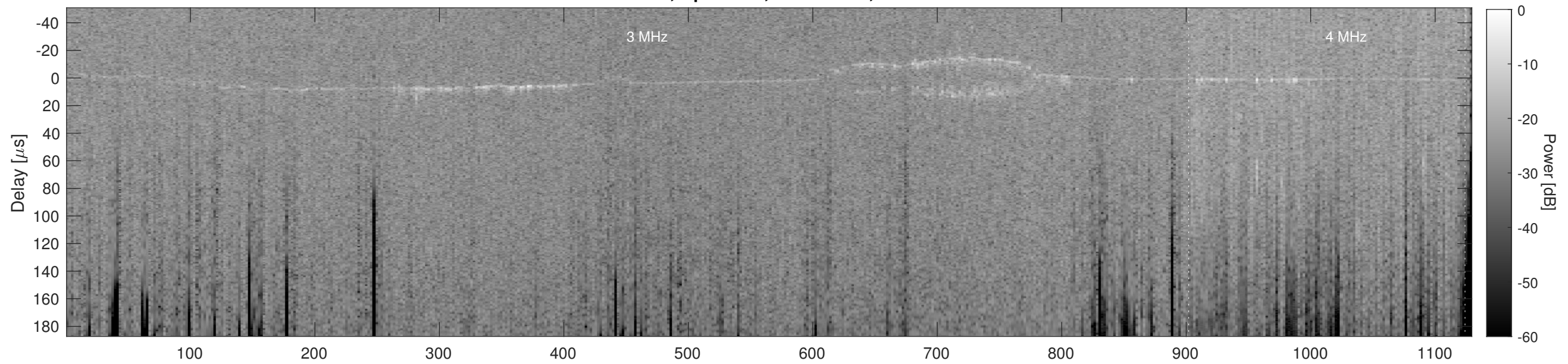
Orbit 11965, Cluttergram
