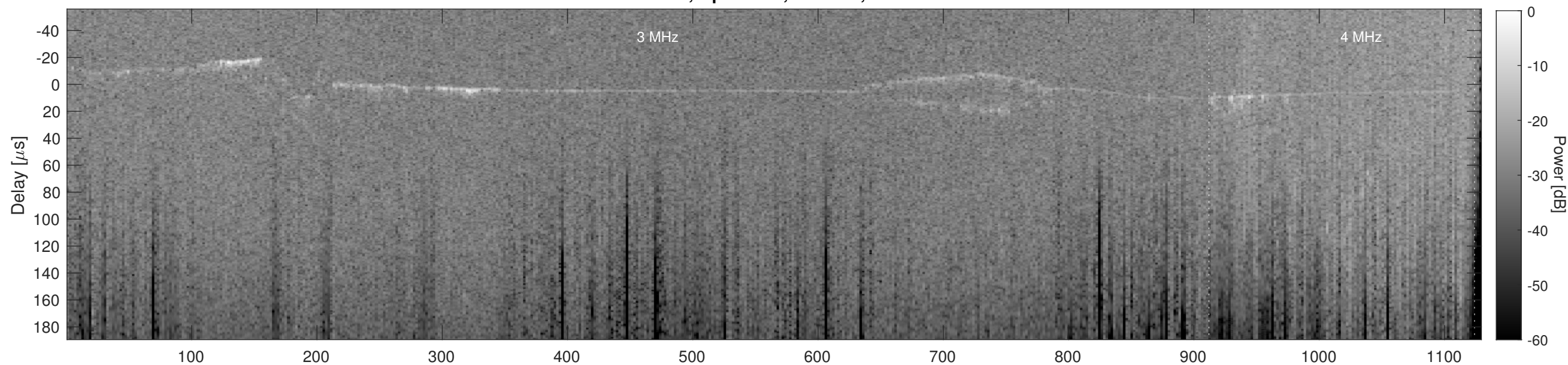
Orbit 11968, Cluttergram
