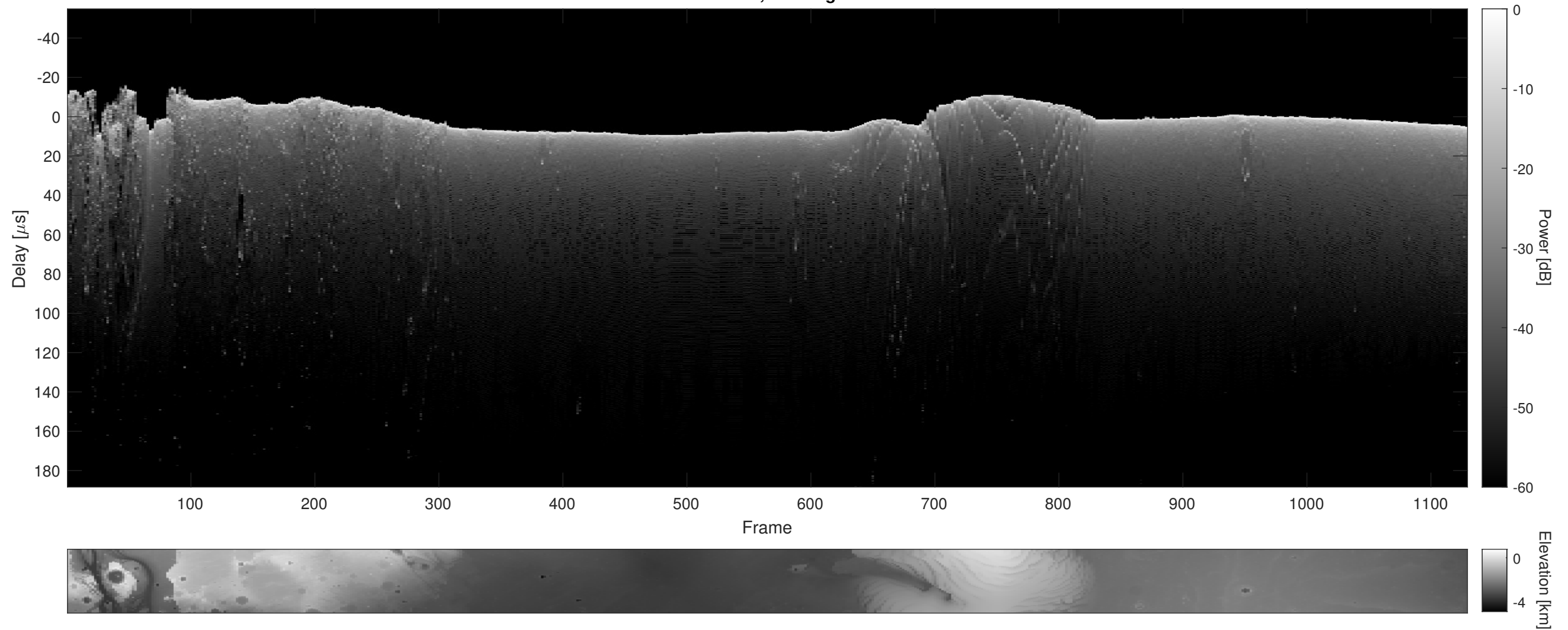
Orbit 11969, Cluttergram
