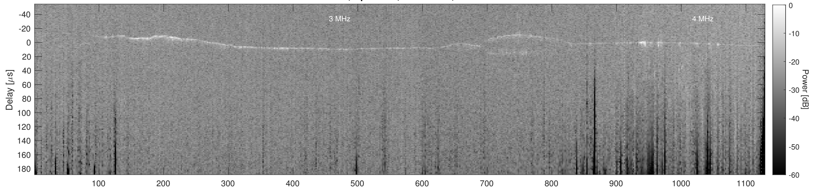
Orbit 11969, Cluttergram
