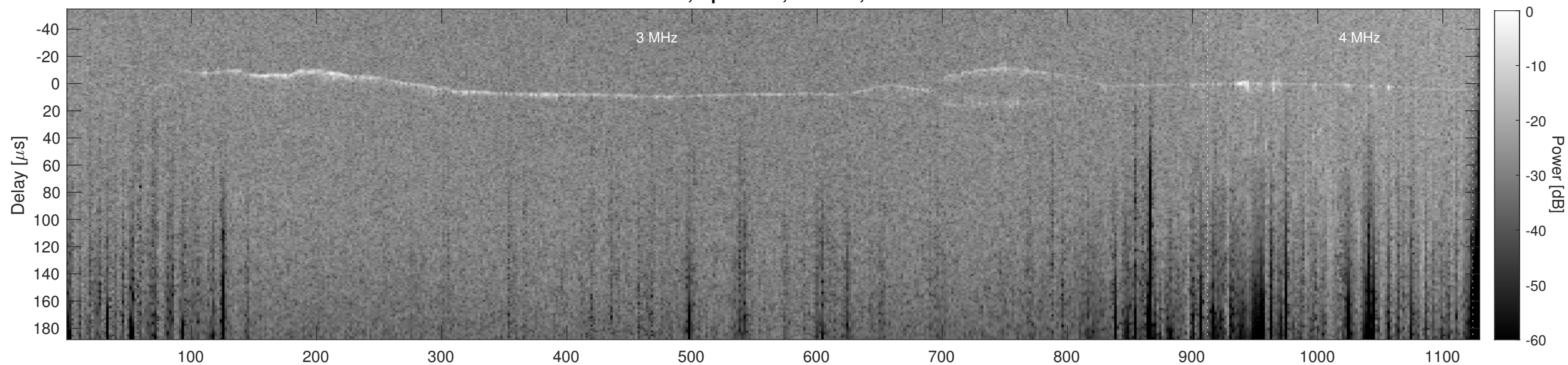
Orbit 11969, Cluttergram
