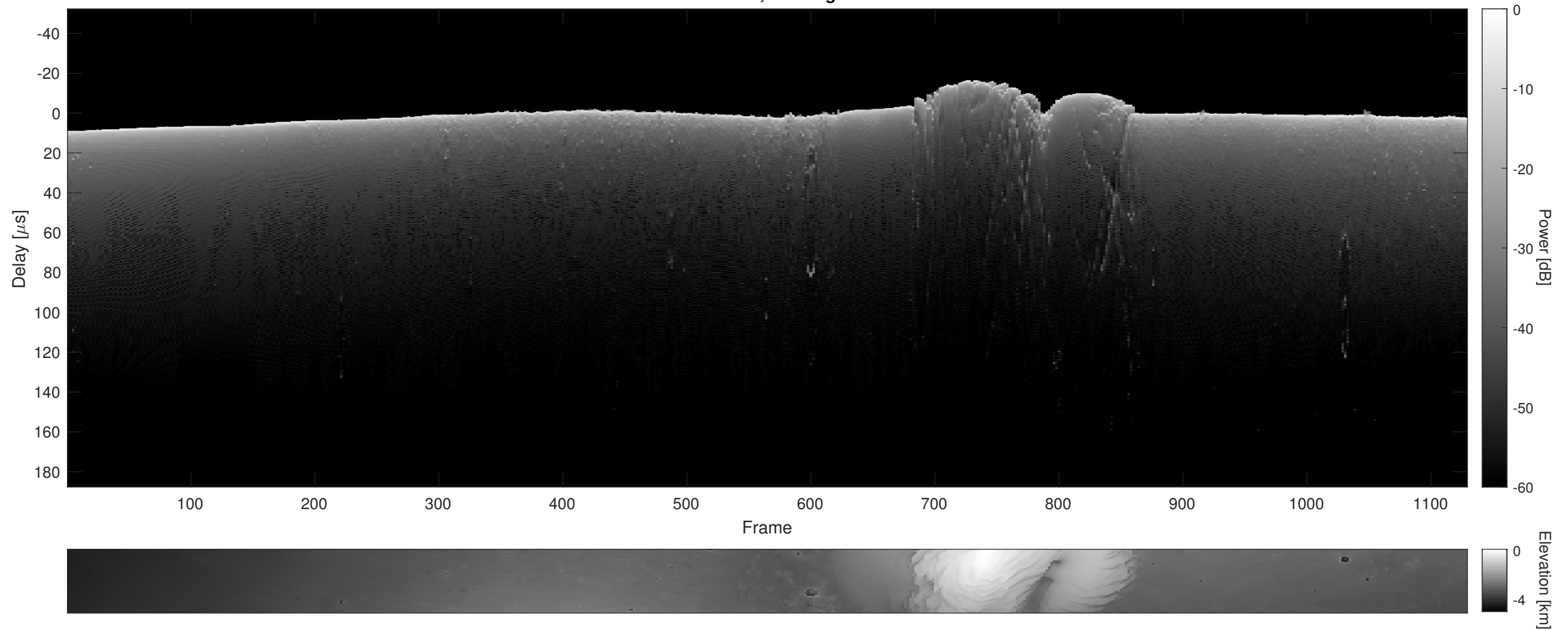
Orbit 11970, Cluttergram
