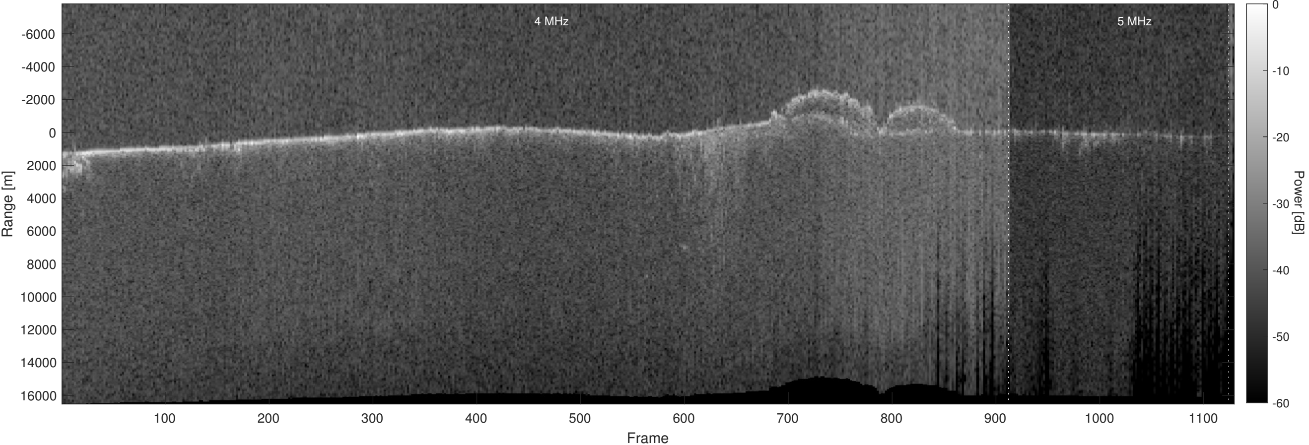
Orbit 11970, Optimized, Window, Depth-Corrected, Channel 2
