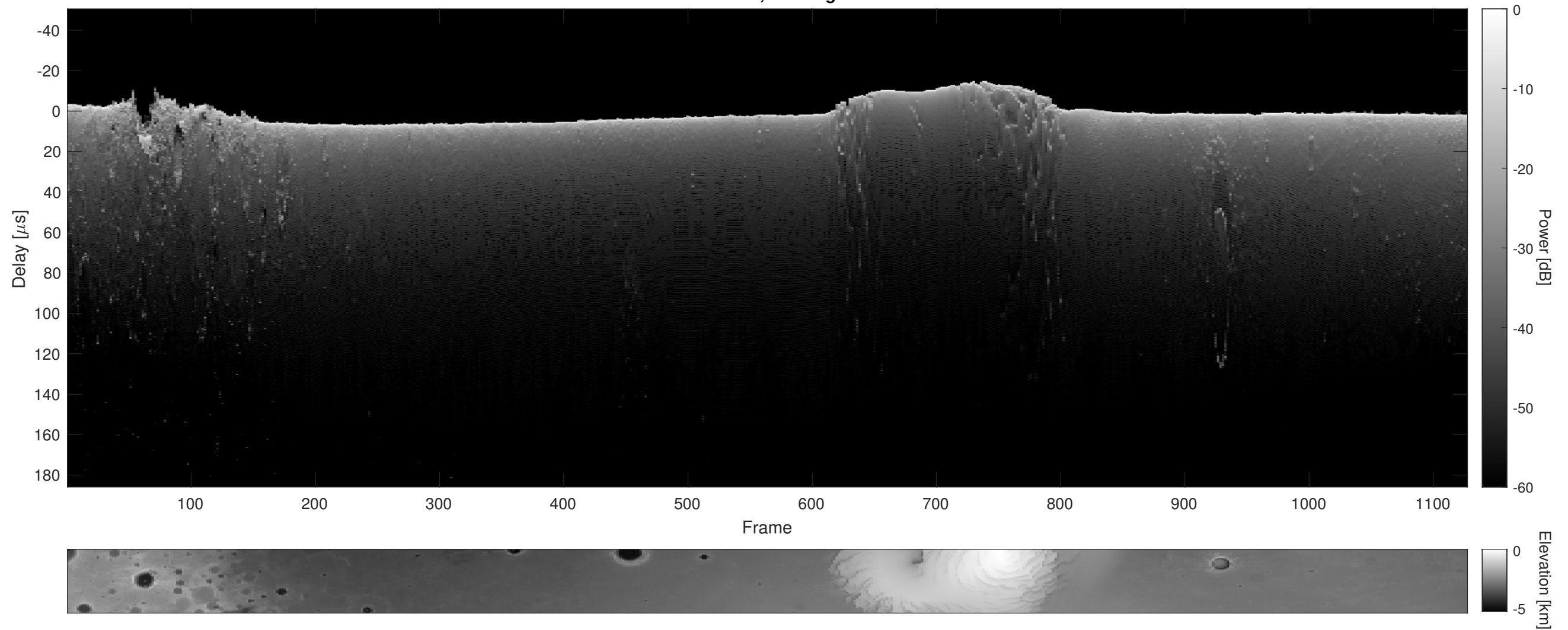
Orbit 11972, Cluttergram
