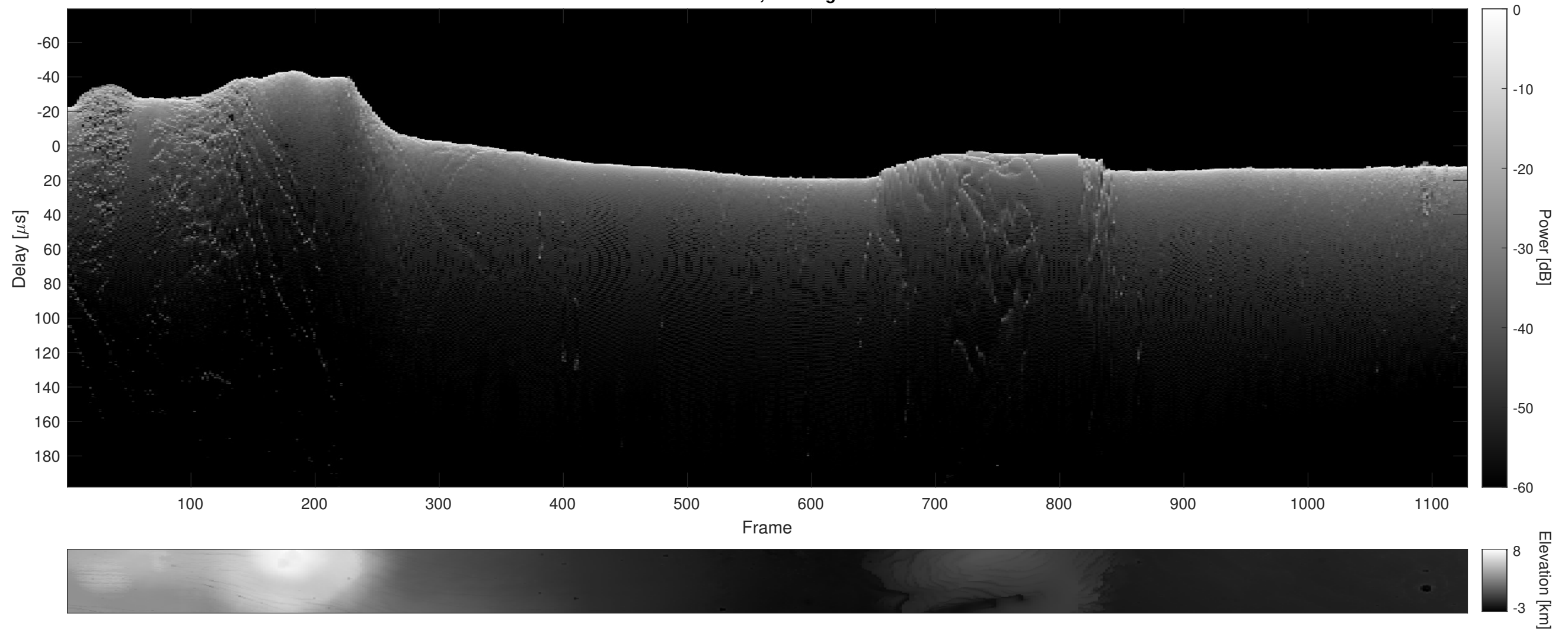
Orbit 11973, Cluttergram
