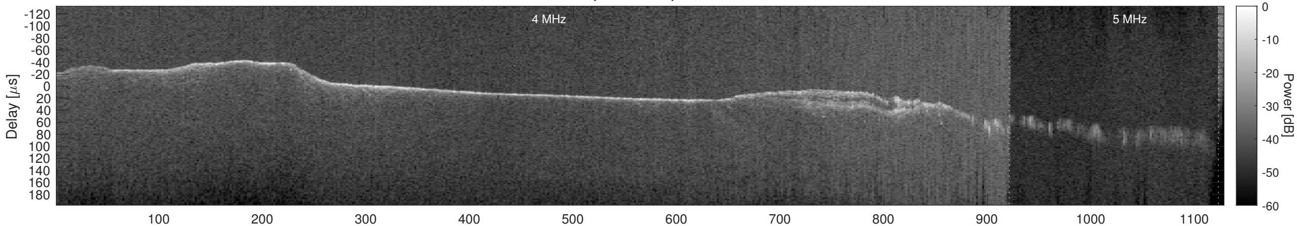
Orbit 11973, Window, Channel 1, Chapman
