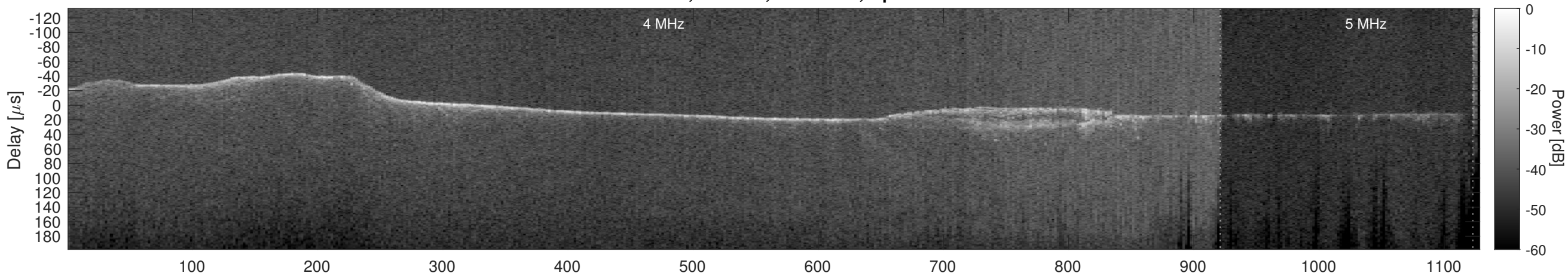
Orbit 11973, Cluttergram
