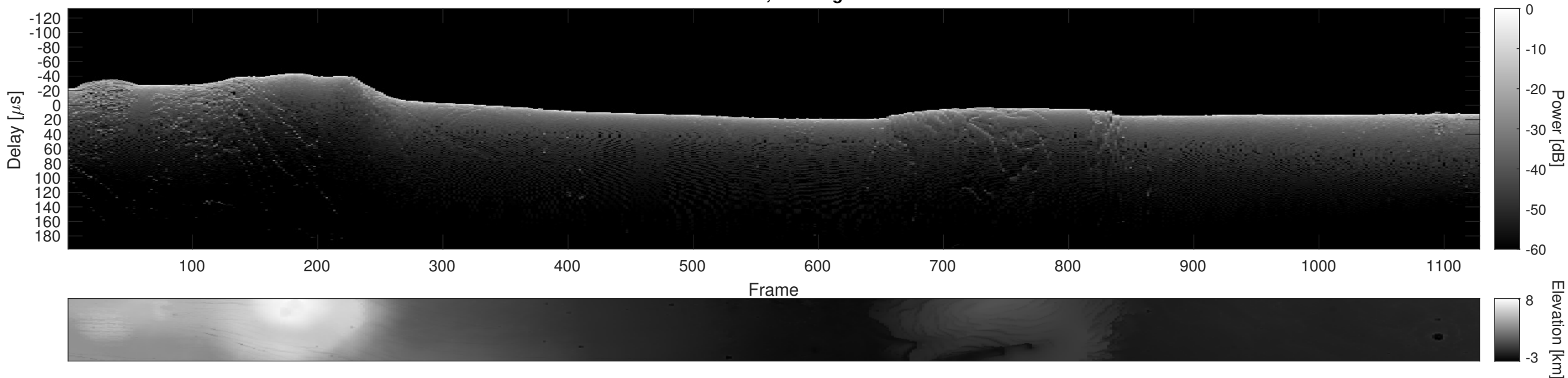
Orbit 11973, Cluttergram
