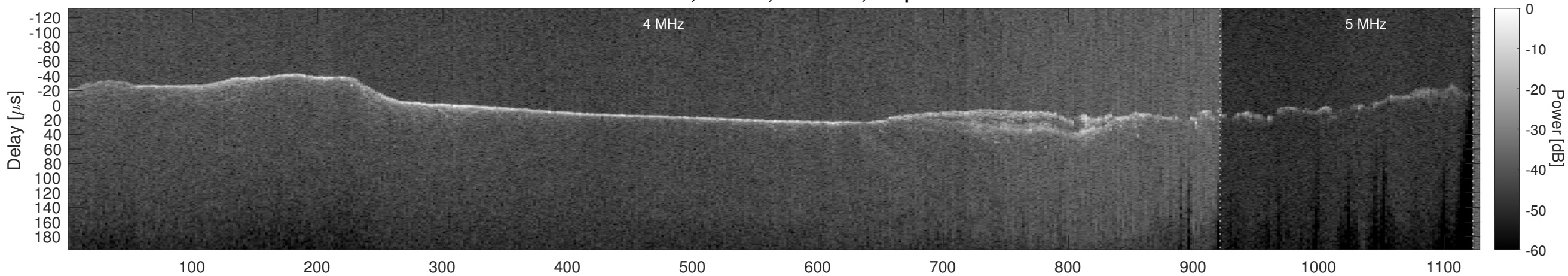
Orbit 11973, Window, Channel 1, Optimized
