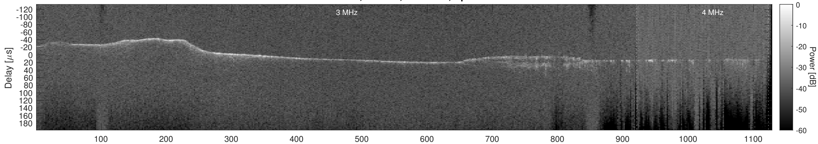
Orbit 11973, Cluttergram
