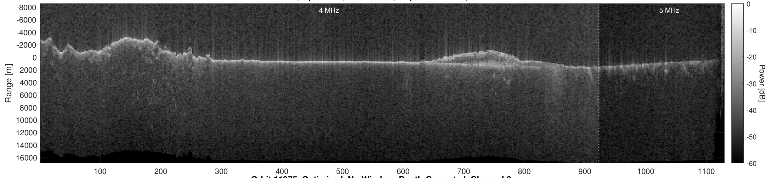
Orbit 11975, Optimized, No Window, Depth-Corrected, Channel 2
