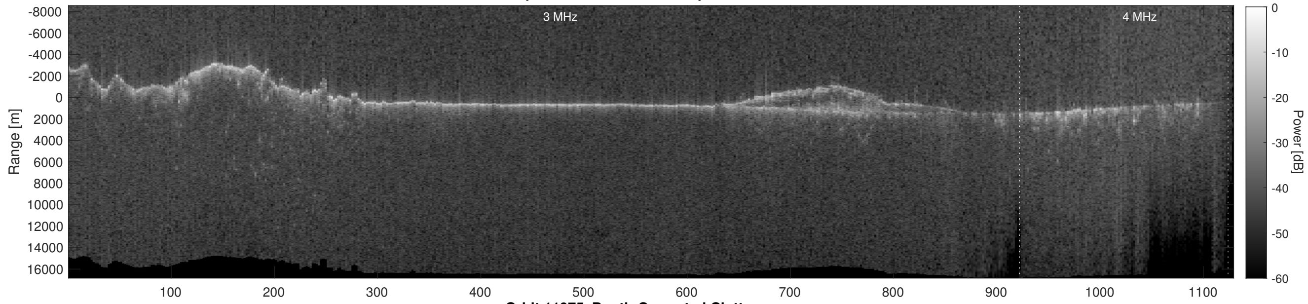
Orbit 11975, Depth-Corrected Cluttergram
