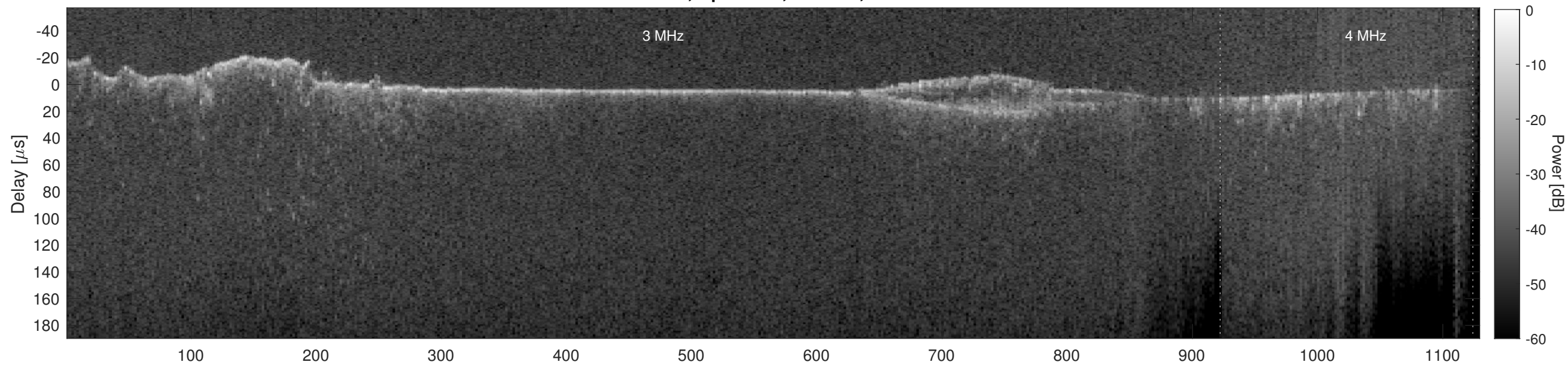
Orbit 11975, Cluttergram
