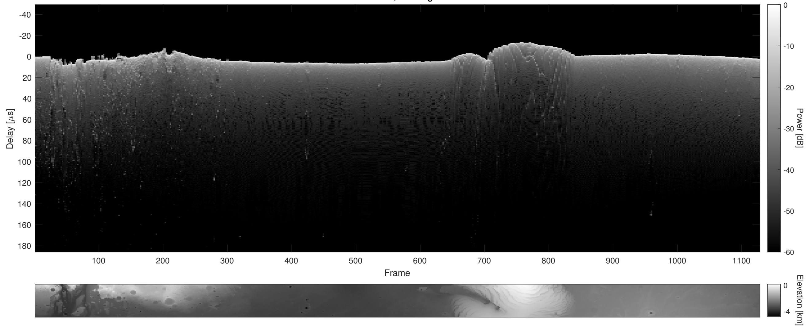
Orbit 11976, Cluttergram
