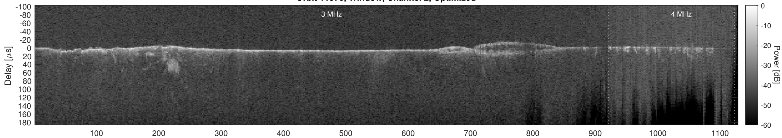
Orbit 11976, Cluttergram
