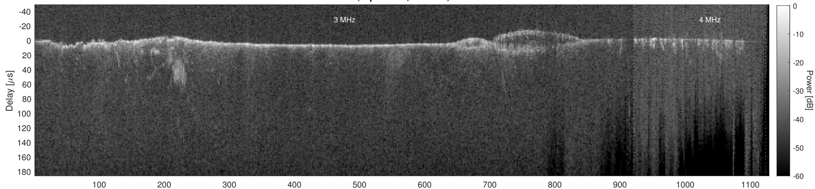
Orbit 11976, Cluttergram
