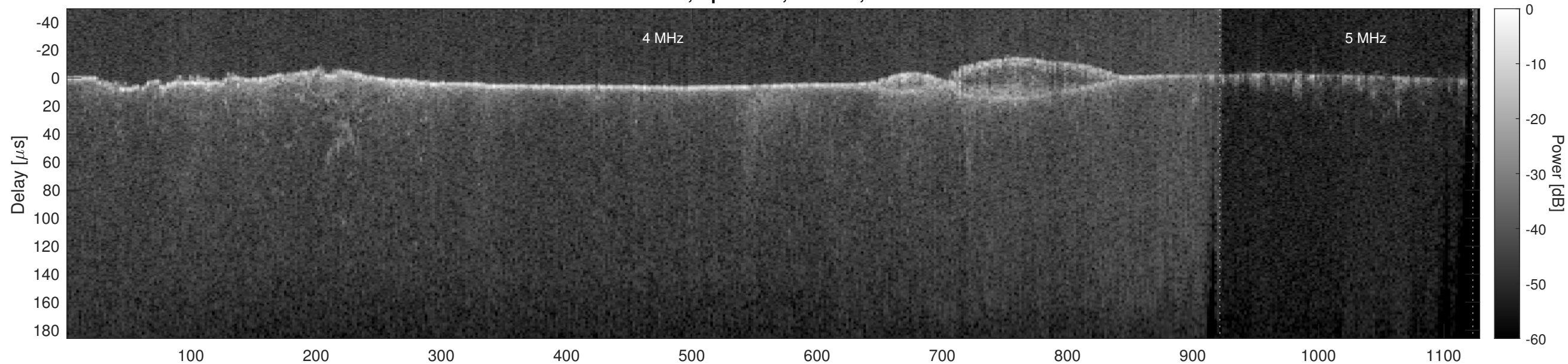
Orbit 11976, Optimized, Window, Channel 2
