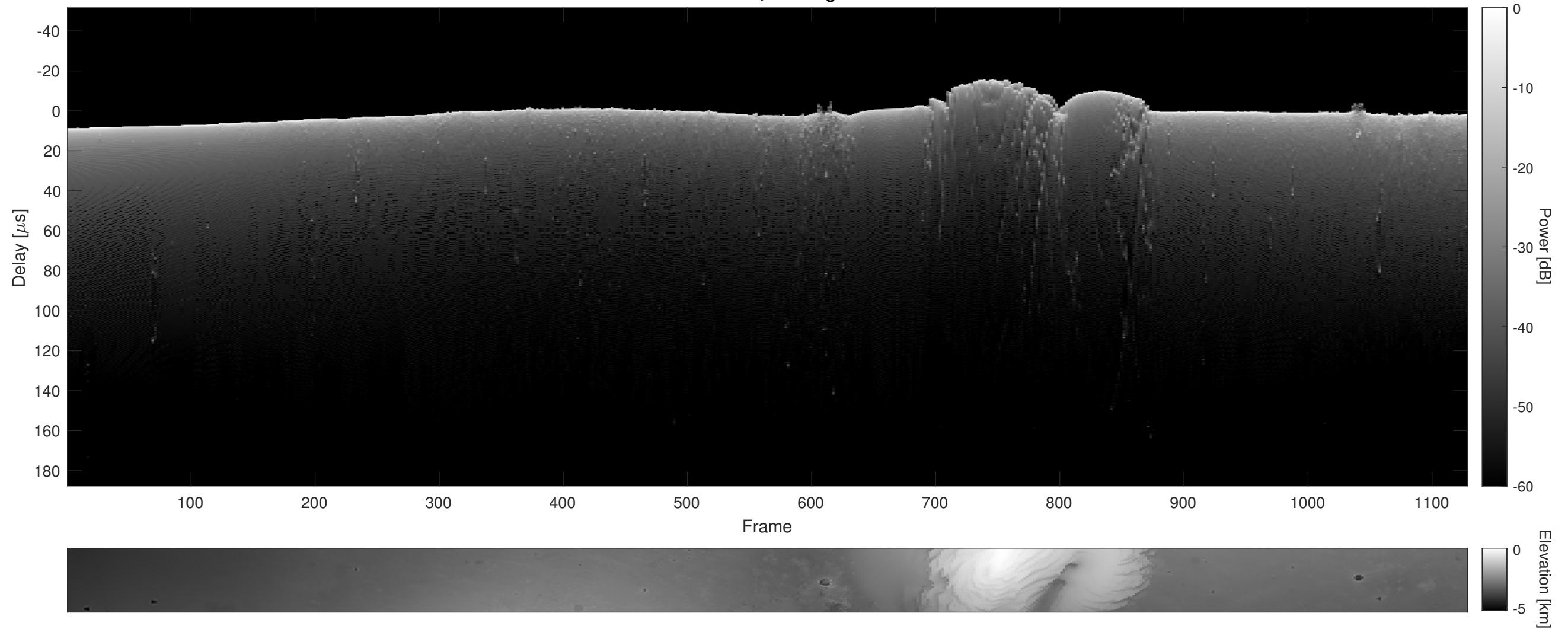
Orbit 11977, Cluttergram
