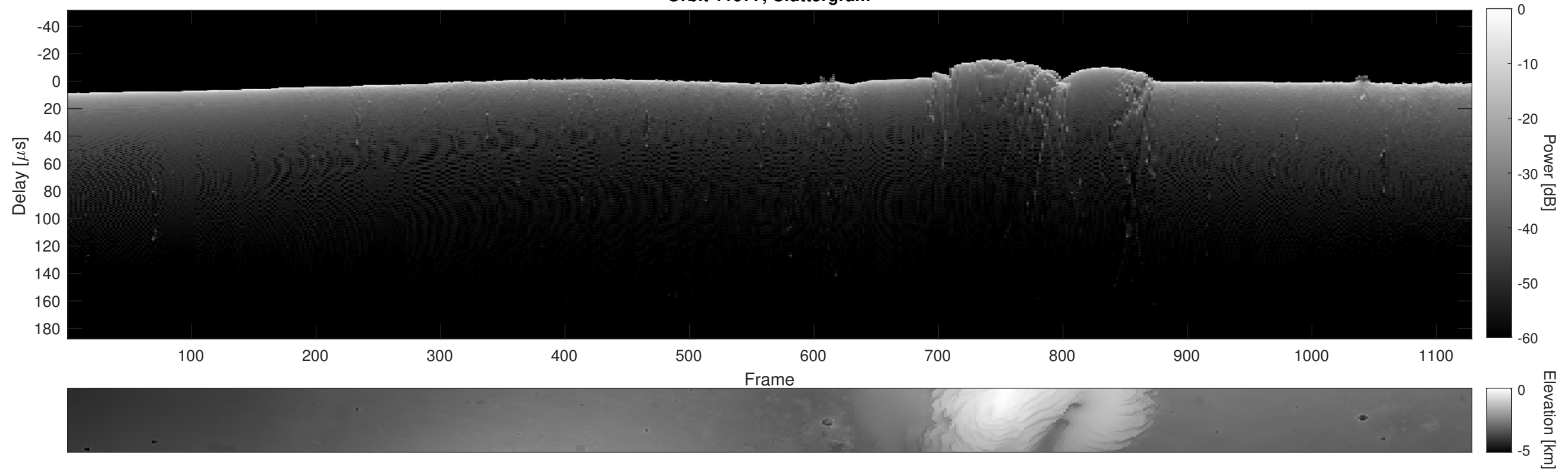
Orbit 11977, Cluttergram
