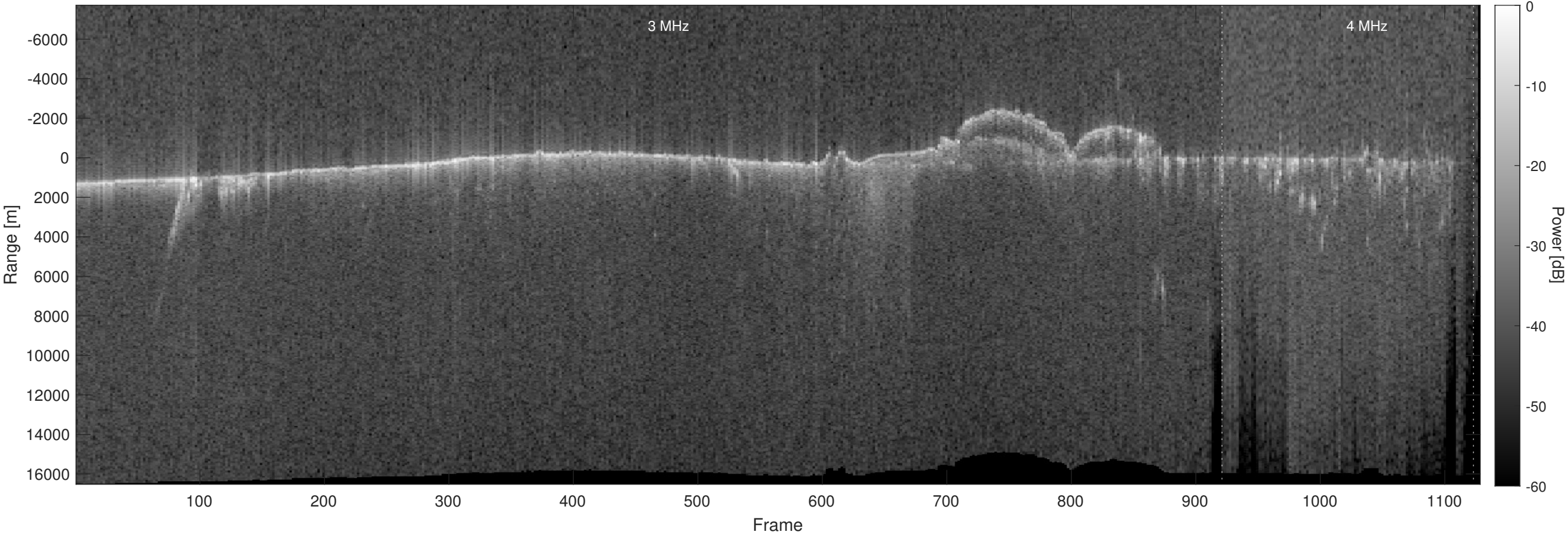
Orbit 11977, Optimized, No Window, Depth-Corrected, Channel 2
