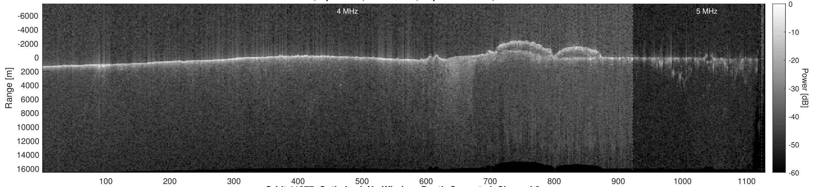
Orbit 11977, Optimized, No Window, Depth-Corrected, Channel 2
