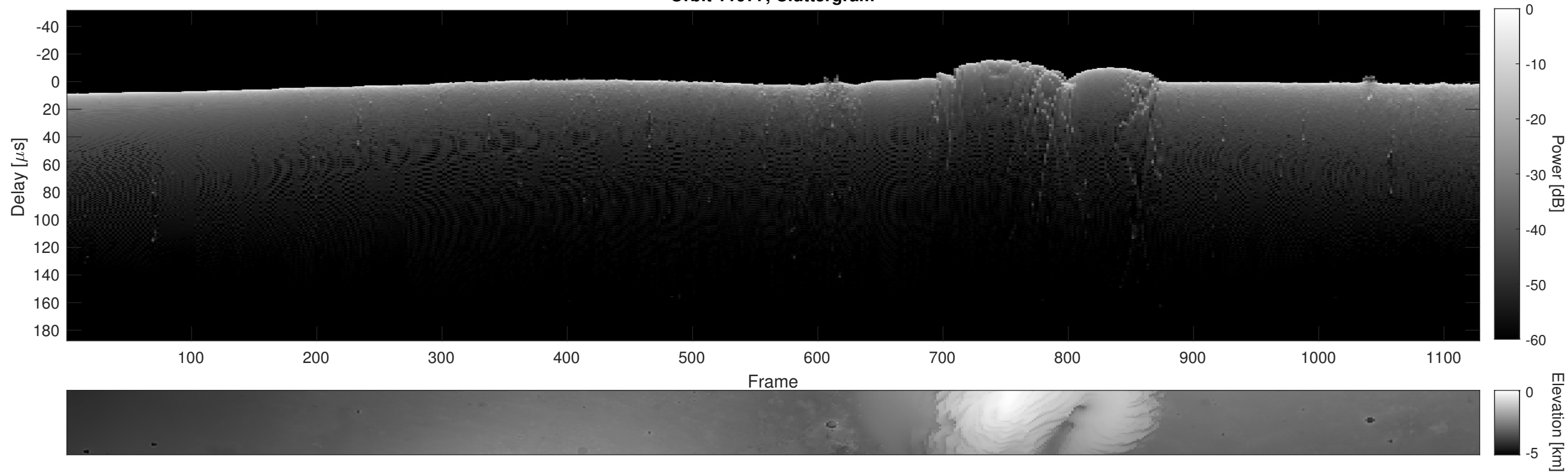
Orbit 11977, Cluttergram
