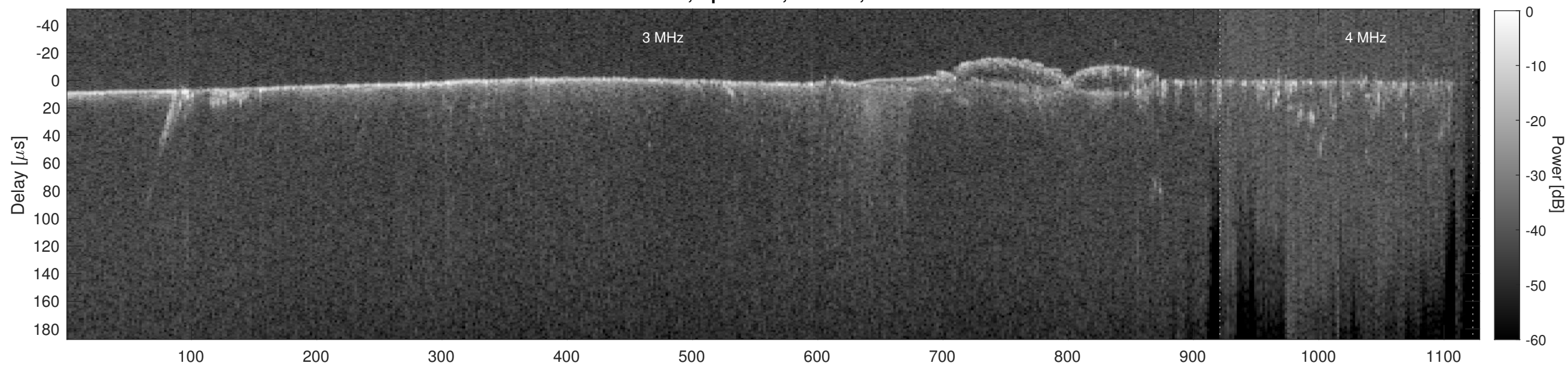
Orbit 11977, Cluttergram
