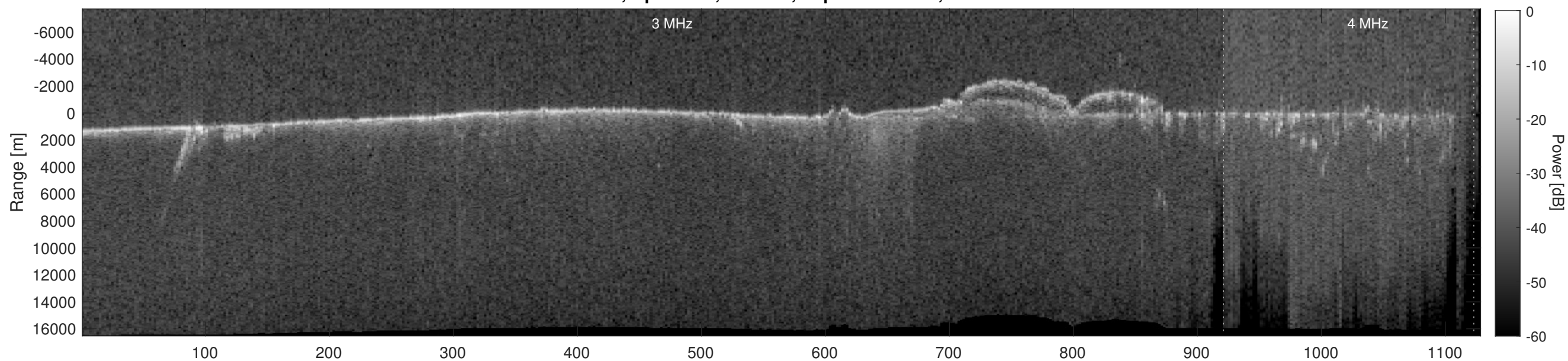
Orbit 11977, Depth-Corrected Cluttergram
