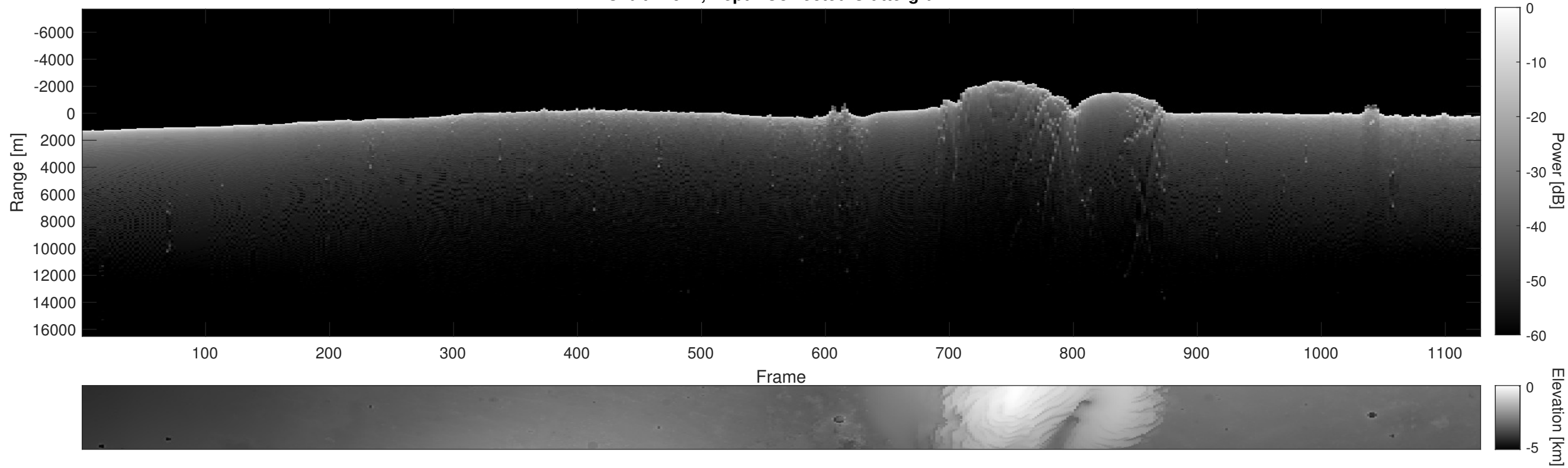
Orbit 11977, Depth-Corrected Cluttergram
