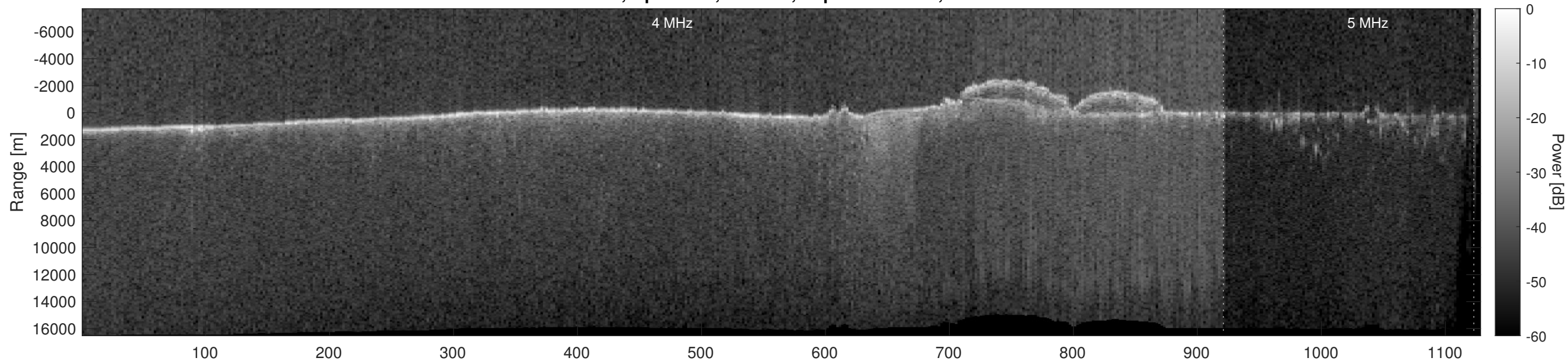
Orbit 11977, Optimized, Window, Depth-Corrected, Channel 2
