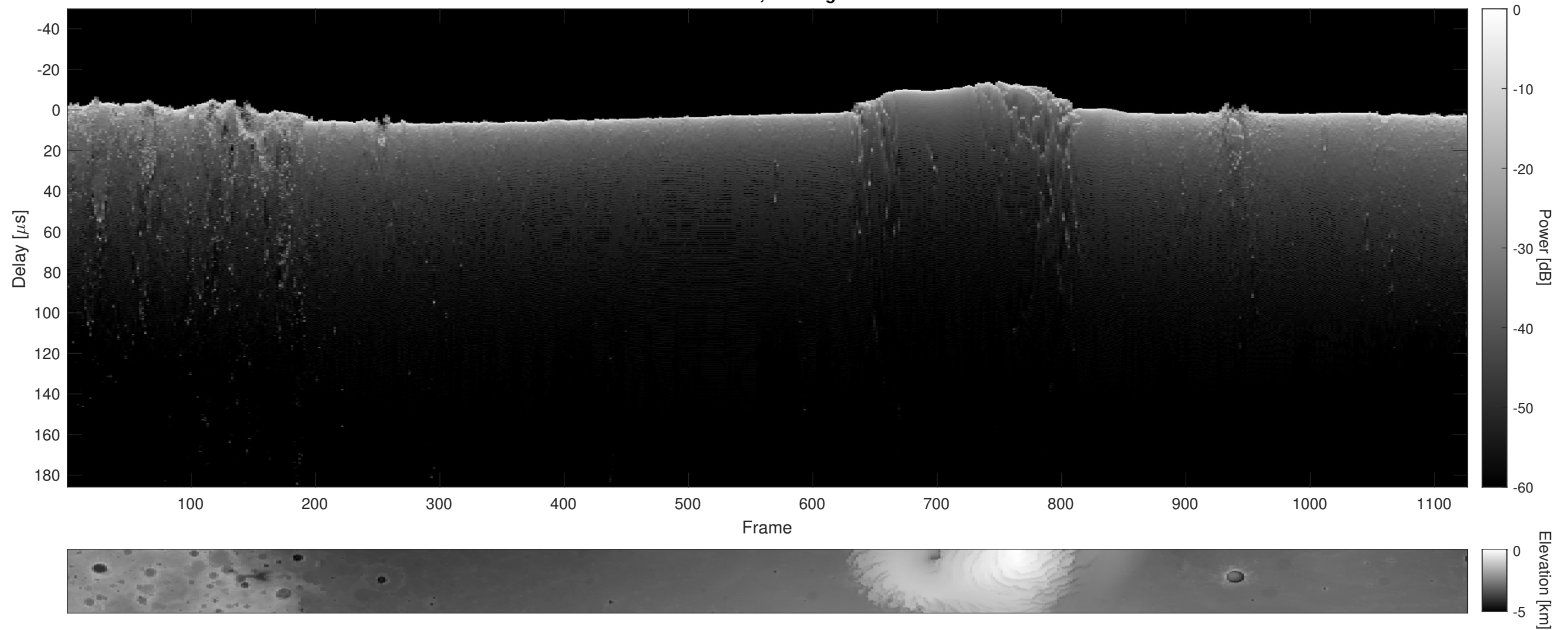
Orbit 11979, Cluttergram
