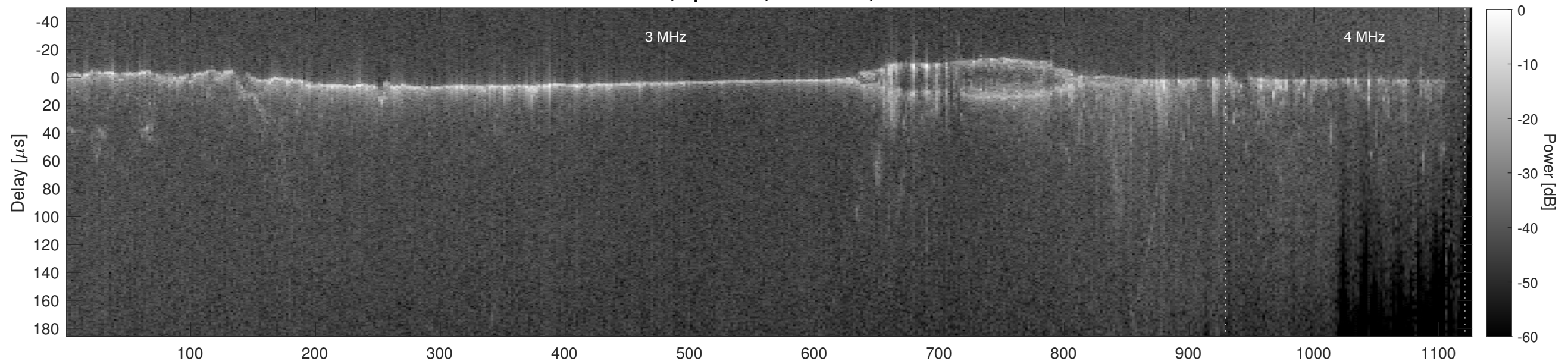
Orbit 11979, Cluttergram
