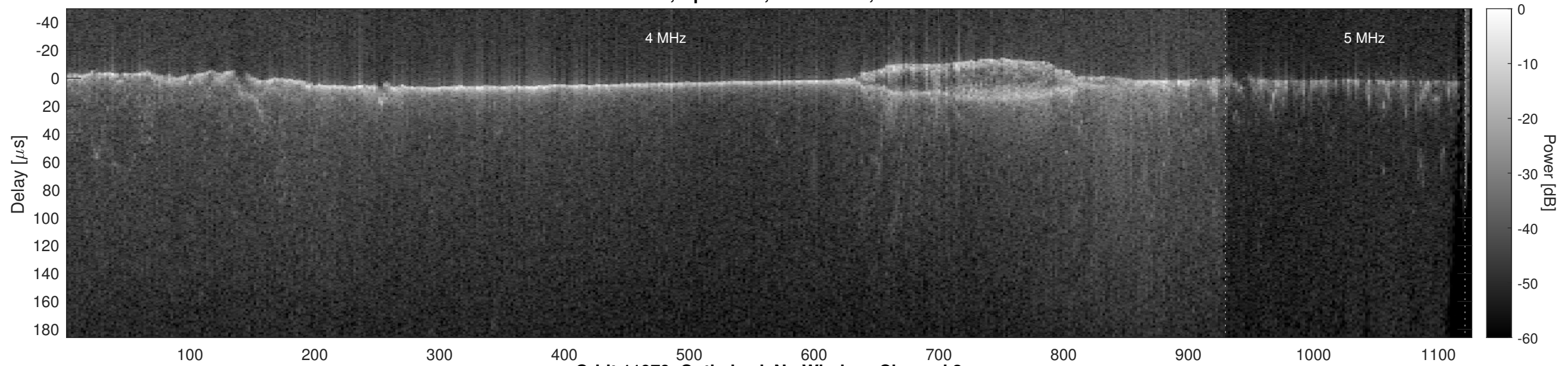
Orbit 11979, Optimized, No Window, Channel 2
