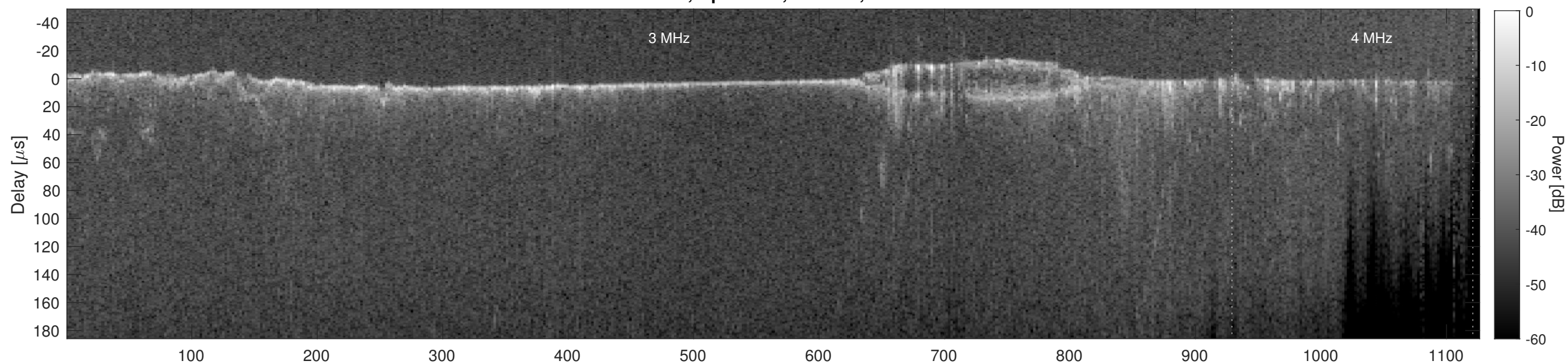
Orbit 11979, Cluttergram
