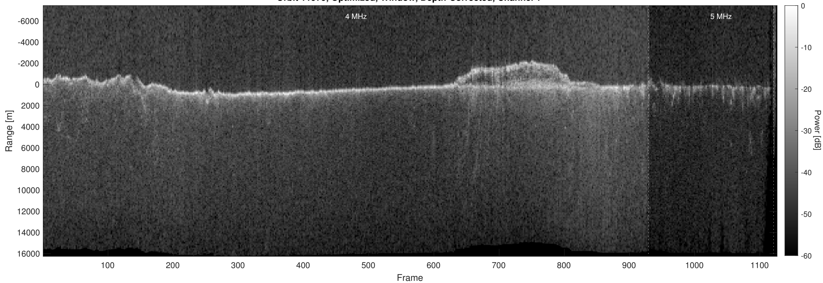
Orbit 11979, Optimized, Window, Depth-Corrected, Channel 2
