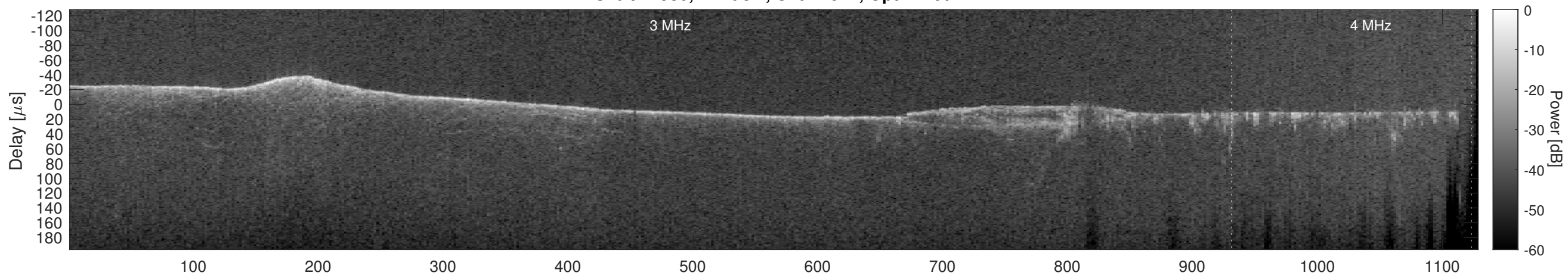
Orbit 11980, Cluttergram
