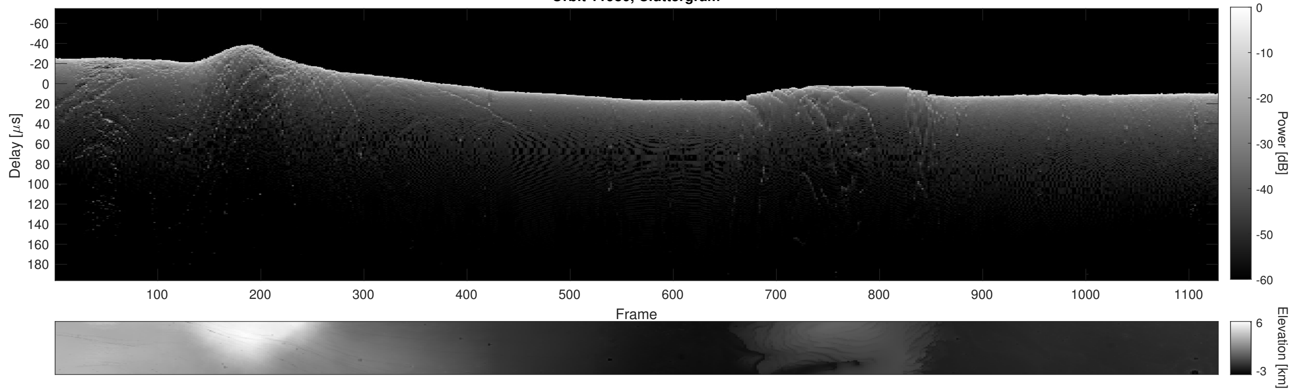
Orbit 11980, Cluttergram
