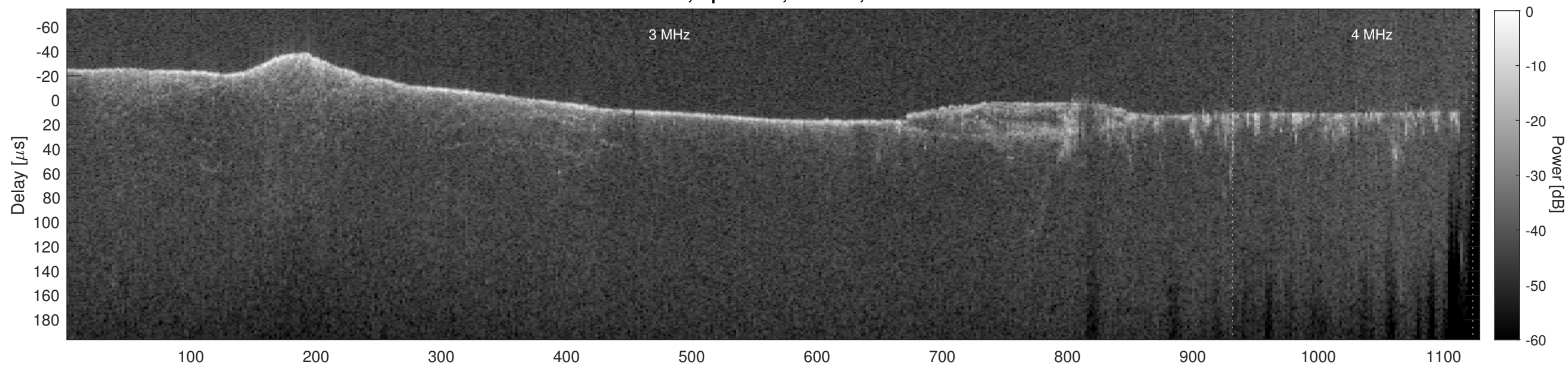
Orbit 11980, Cluttergram
