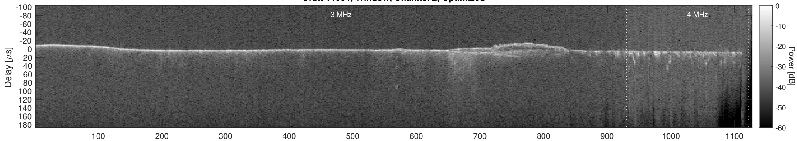
Orbit 11981, Cluttergram
