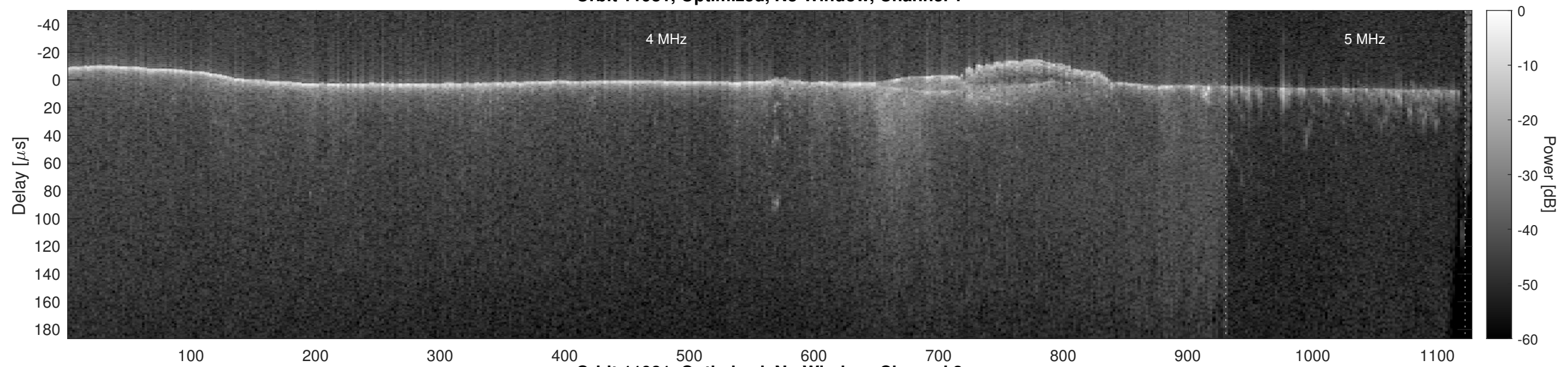
Orbit 11981, Optimized, No Window, Channel 2
