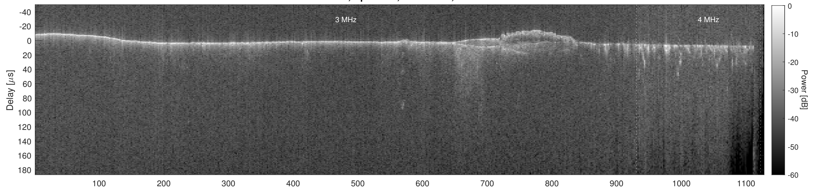
Orbit 11981, Cluttergram
