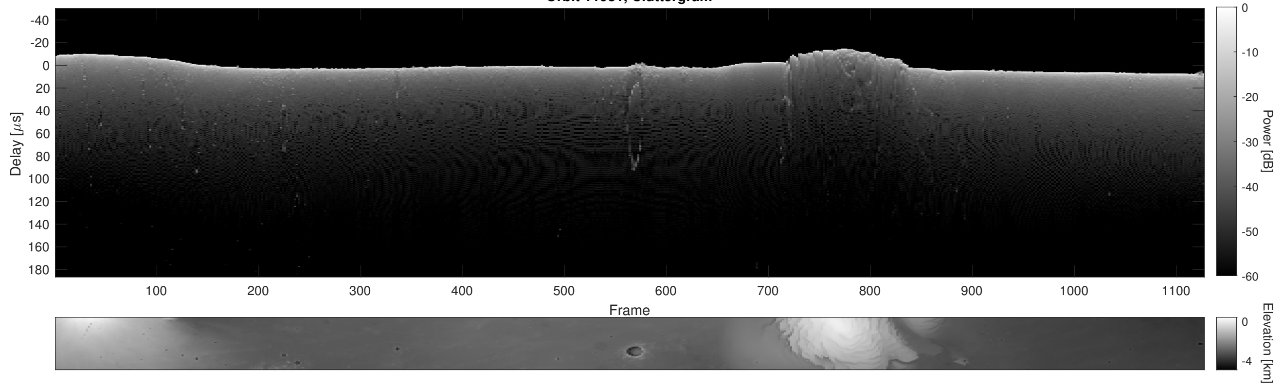
Orbit 11981, Cluttergram
