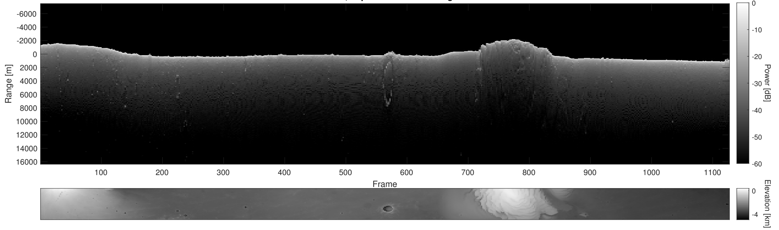
Orbit 11981, Depth-Corrected Cluttergram
