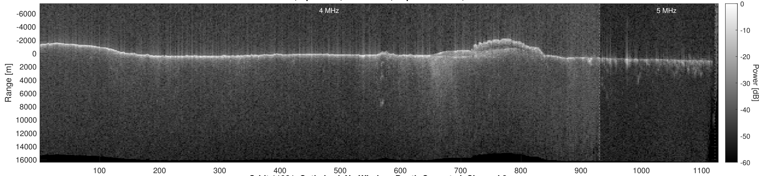
Orbit 11981, Optimized, No Window, Depth-Corrected, Channel 2
