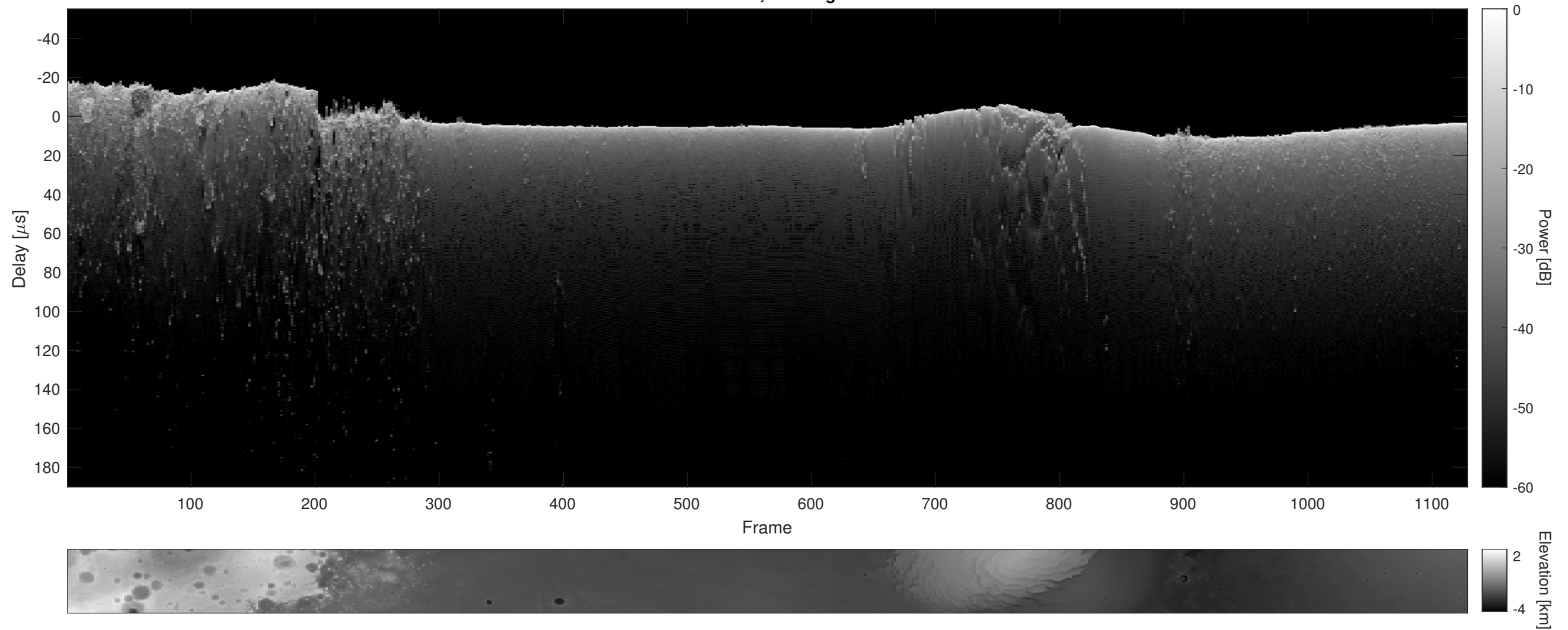
Orbit 11982, Cluttergram
