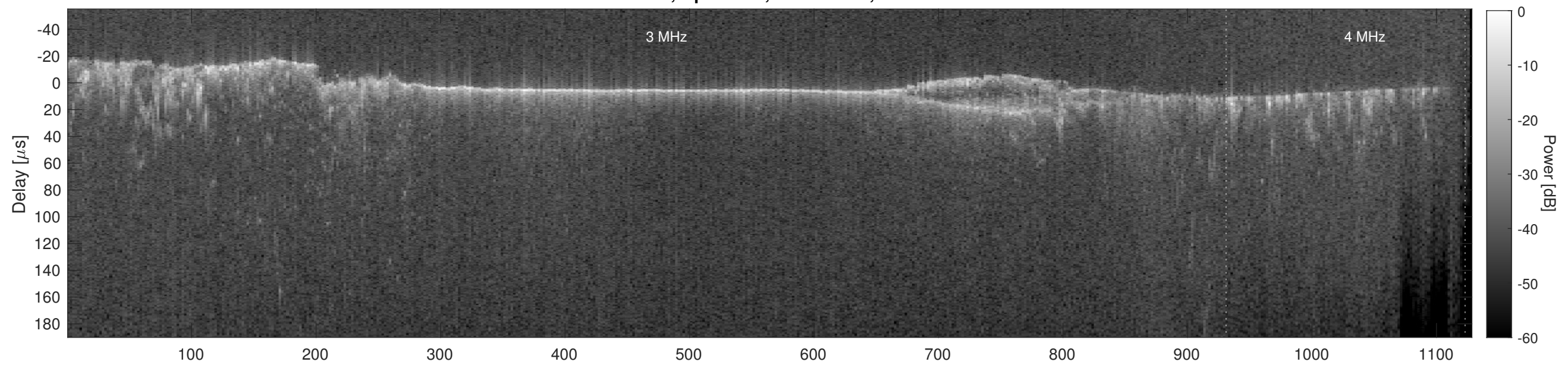
Orbit 11982, Cluttergram
