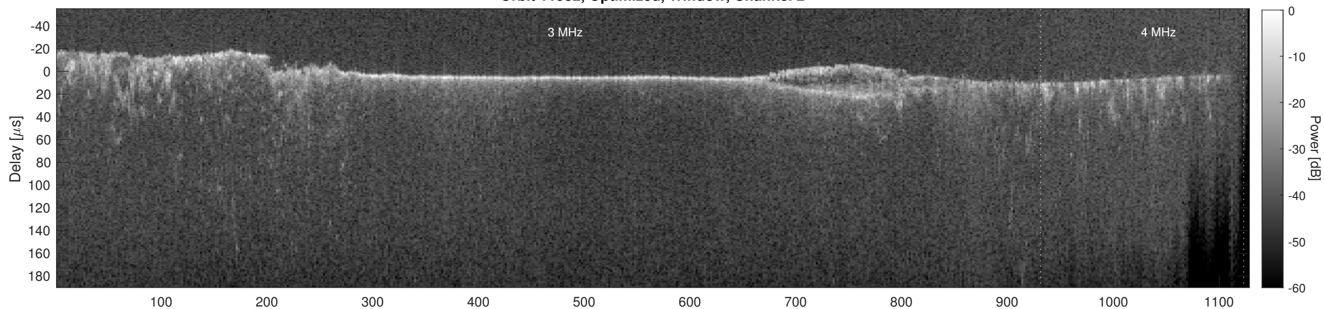
Orbit 11982, Cluttergram
