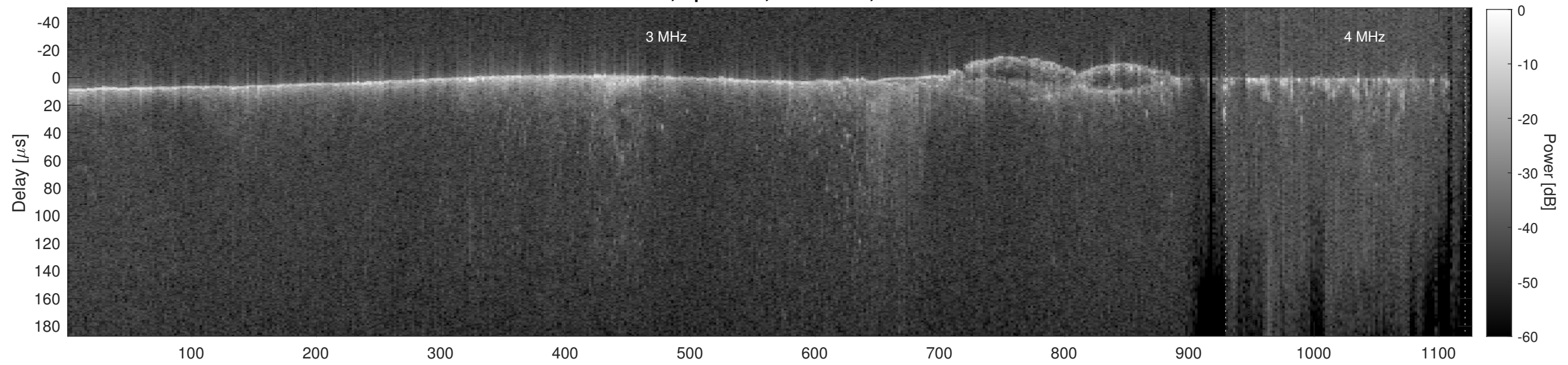
Orbit 11984, Cluttergram
