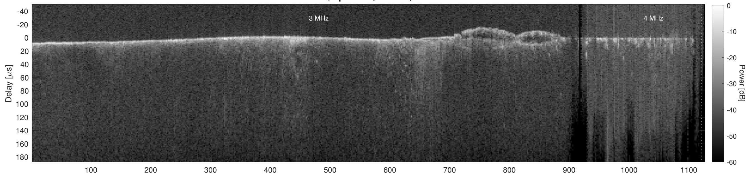
Orbit 11984, Cluttergram
