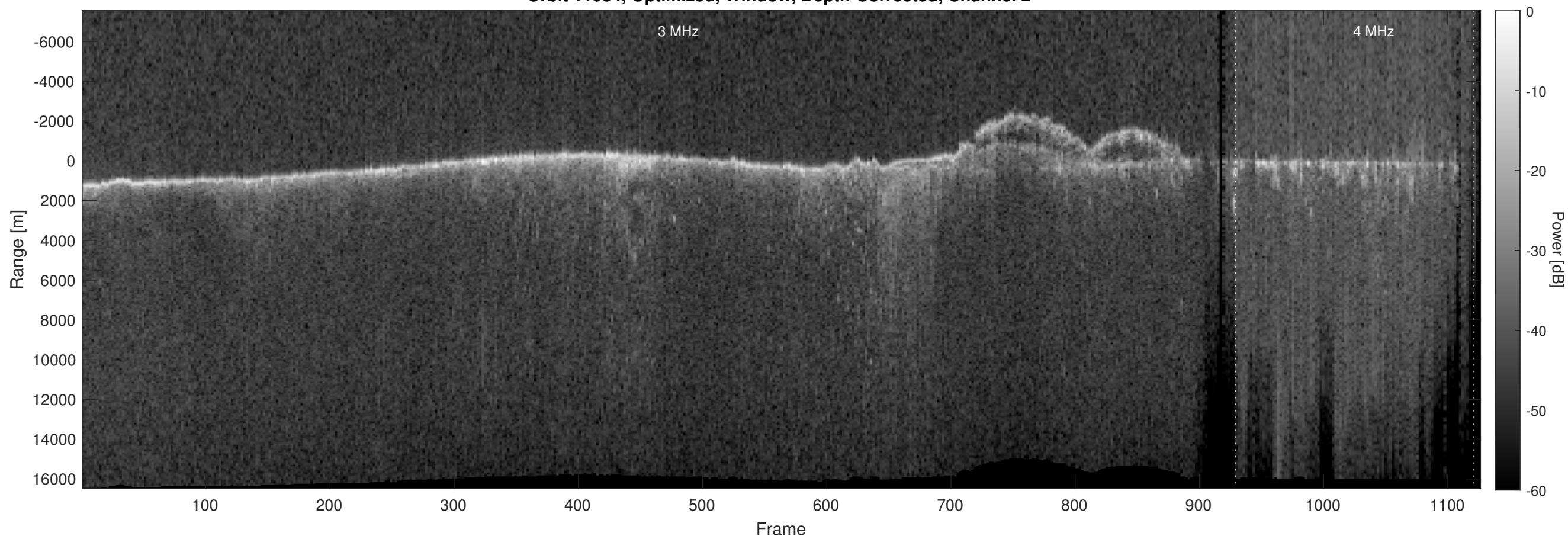
Orbit 11984, Optimized, Window, Depth-Corrected, Channel 2
