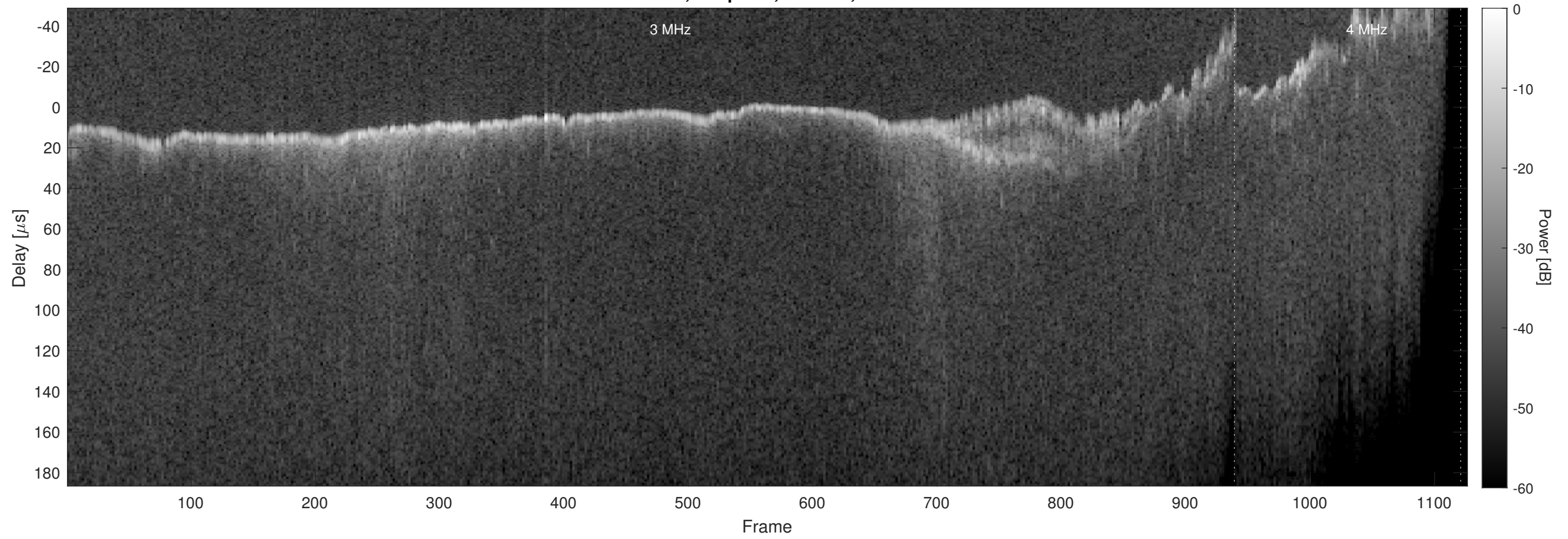
Orbit 11985, Chapman, Window, Channel 2
