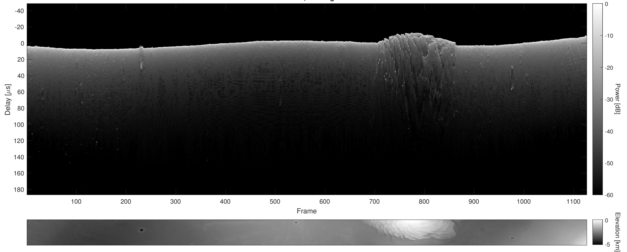
Orbit 11985, Cluttergram
